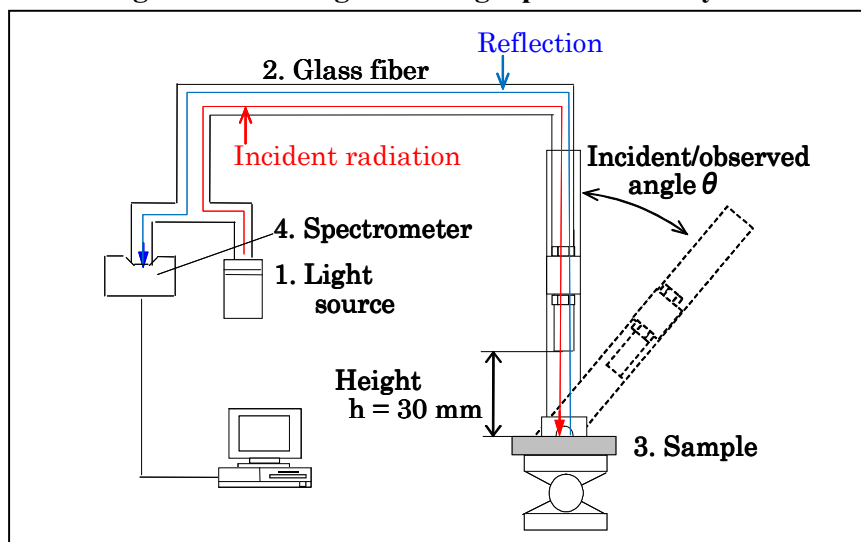
Figure 2. Emitting-Receiving Optical Fiber System
